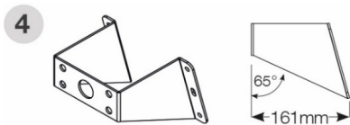
Wall Brackets
