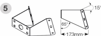
Corner Brackets
